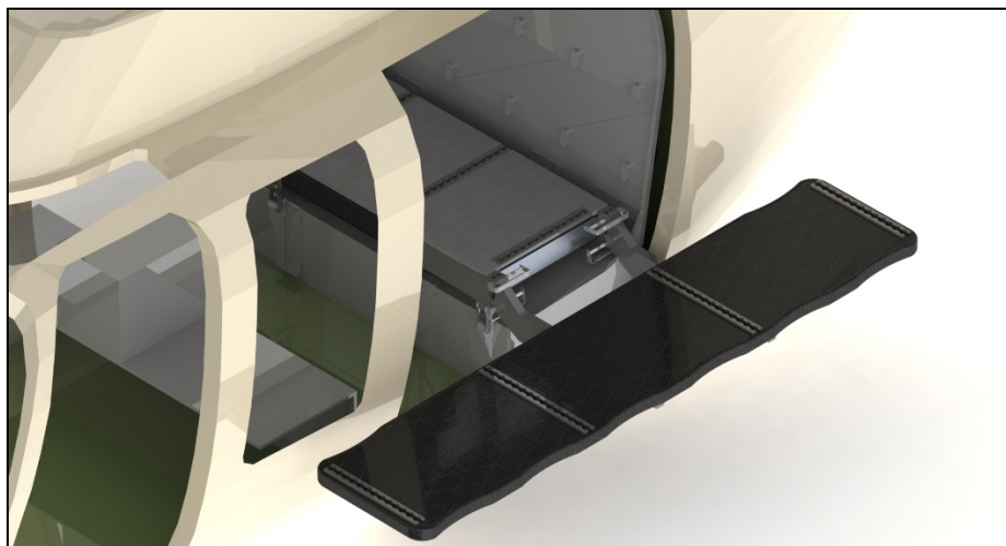
Tactical Assault Bench (TAB) on the BELL 407 Series II ALWiP
